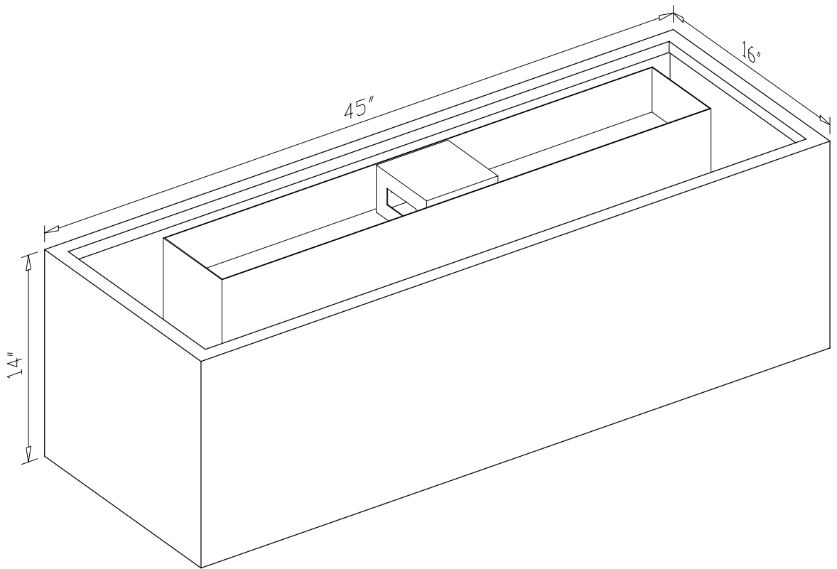
Prosperity 1 Tank 45"L x 16" D x 14"H
